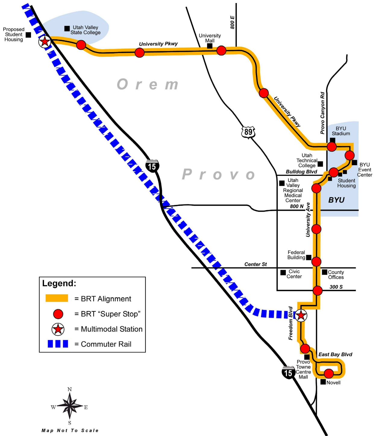
Figure ES-3 Bus Rapid Transit Schematic
